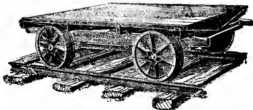
Fig. 5601. Perspective View. THE BUDA PUSH-CAR No. 6. Platform, 7 ft. \times 5½ ft. Weight, 450 lbs.
